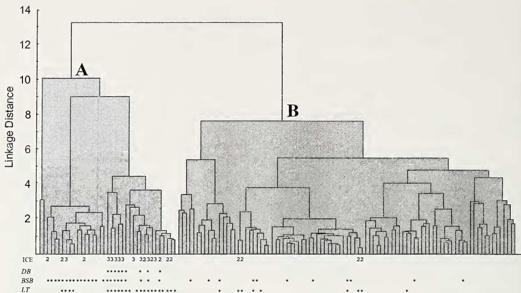
Figure 2.—Spider communities in Czech screes, as revealed by a cluster analysis of samples. The A and B clusters were supported by bootstrap resampling. ICE = ice formation (2 = temporal ice inside scree, melting in summer; 3 = permanent ice forming permafrost). Presence of three indicators of ice incidence ( DB = Diplocentria bidentata , BSB = Bathypantes similis buchari , LT = Leptyphantes tripartitus ) is indicated by stars.
